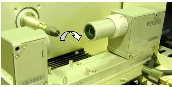
Sample hair is rolled and measured by laser-beam
